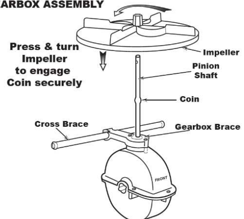
GEARBOX ASSEMBLY
